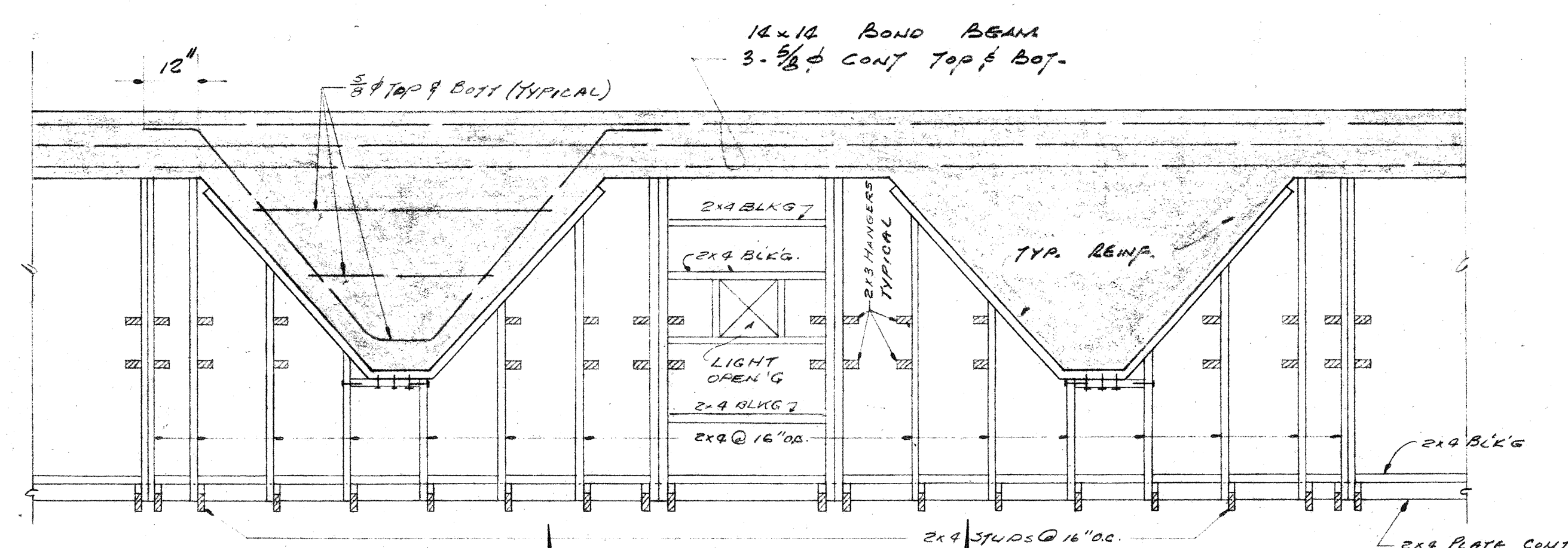
PLAN OF BOND BEAM REINFORCING & LIGHT TROUGH BRACING 1/2" x 1'-0"
