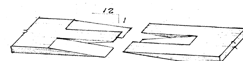
SCARF JOINT SEE SPECIFICATIONS
