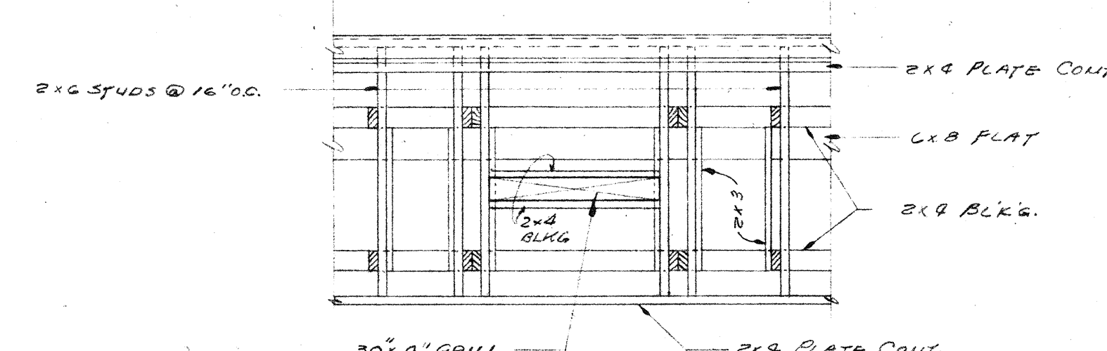
ELEVATION 1 ELEVATION AT EACH GRILL 1/2" x 1'-0"
